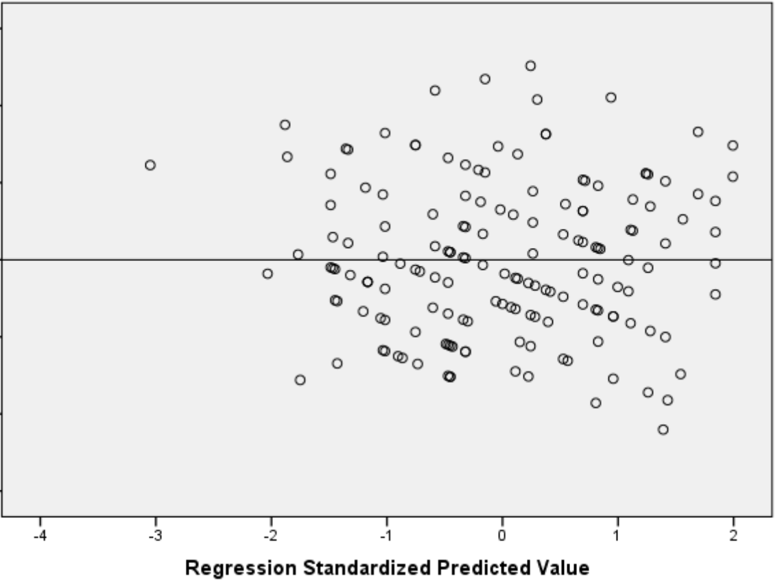
Scatterplot Dependent Variable: PI
