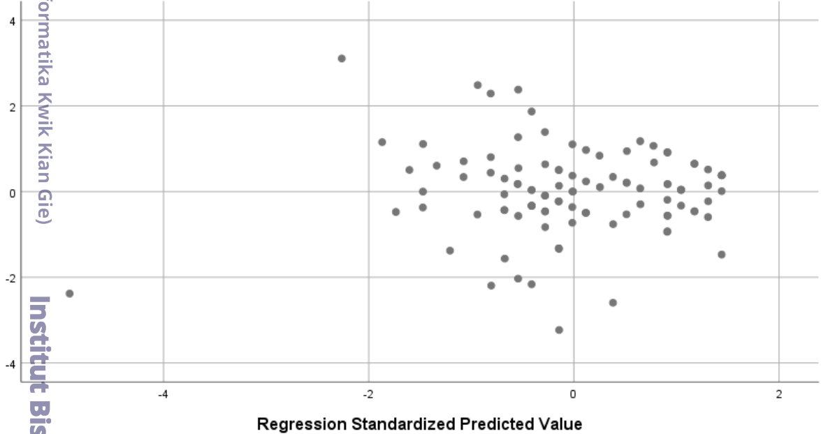
Scatterplot
