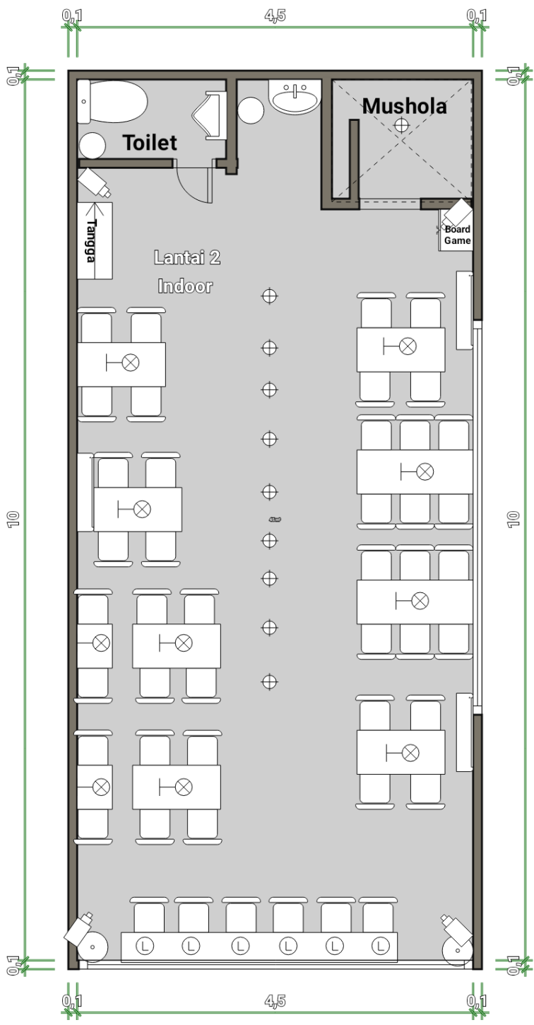
Gambar 5. 11 Layout Meriah Ukur Lantai 2
