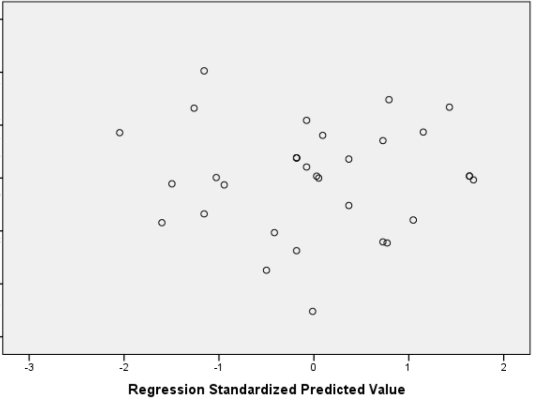
Scatterplot Dependent Variable: Turnover Intention
