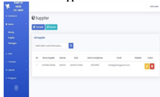
Gambar 10. Halaman Supplier
