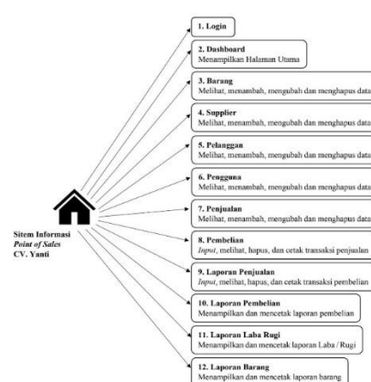
Gambar 6. Sistem Informasi Point of Sales CV. Yanti
