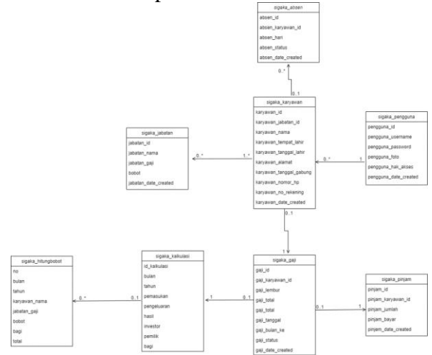
Gambar 4.2 Class Diagram
