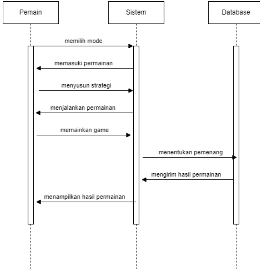
Gambar 6 Sequence diagram memainkan game
