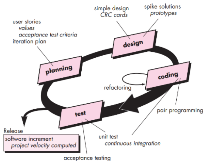
Gambar 1 Extreme Programming Life Cycle
