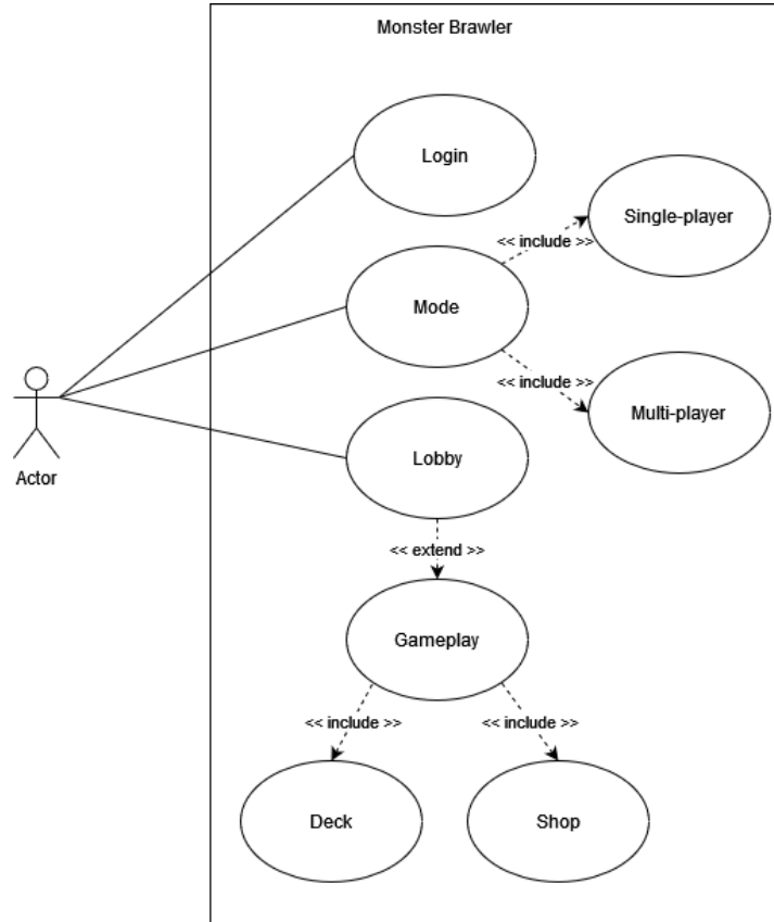
Gambar 3 Use case Diagram Monster Brawler
