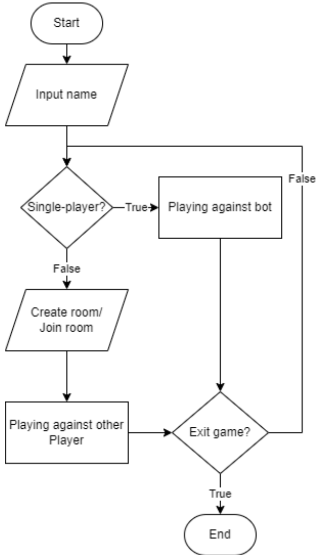
Gambar 5 Flowchart game
