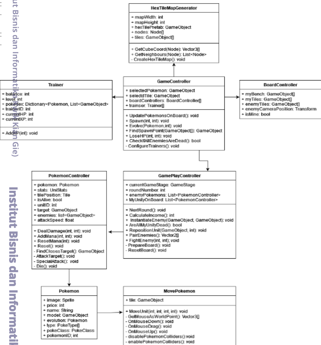
Gambar 7 Class Diagram
