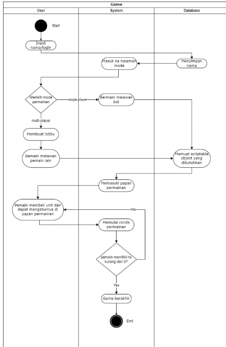
Gambar 4 Activity Diagram
