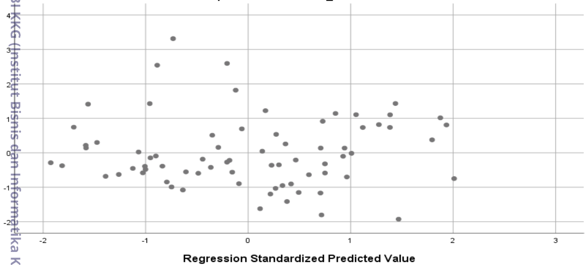
Scatterplot Dependent Variable: Y_PBV
