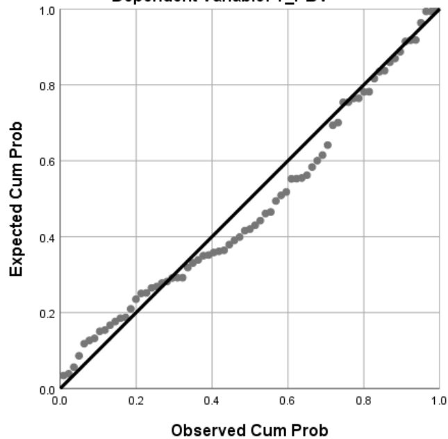
Normal P-P Plot of Regression Standardized Residual Dependent Variable: Y_PBV
