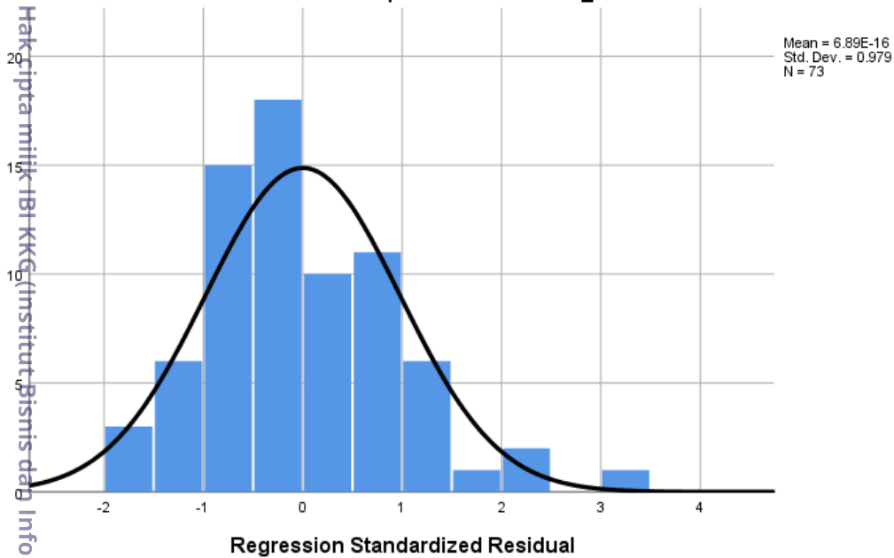
Histogram Dependent Variable: Y_PBV
