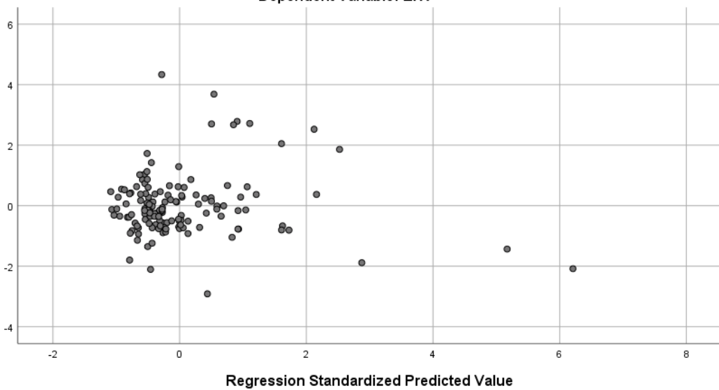
Scatterplot Dependent Variable: EXV
